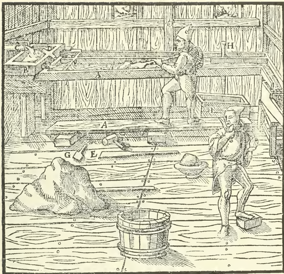
A—STRAKES. B—TANK. C—LAUNDER. D—PLUG. E—WOODEN SHOVEL. F—WOODEN MALLETT. G—WOODEN SHOVEL WITH SHORT HANDLE. H—THE PLUG IN THE STRAKE. I—TANK PLACED UNDER THE PLUG.
